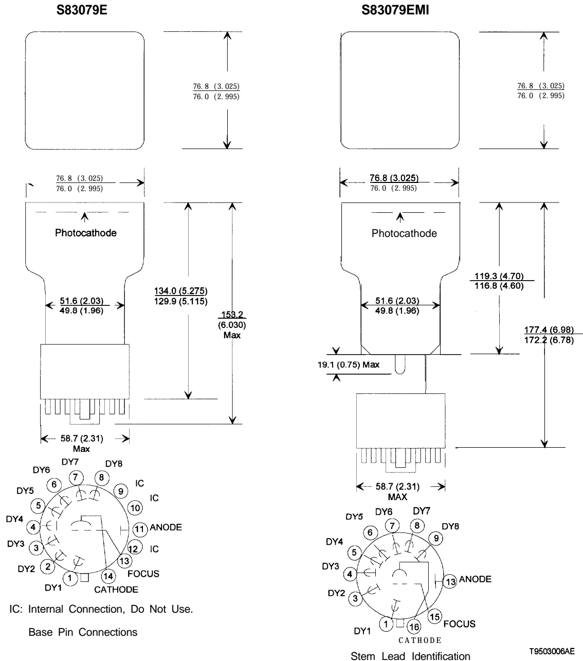
Figure 8: Dimensional Outlines and Basing Diagrams
