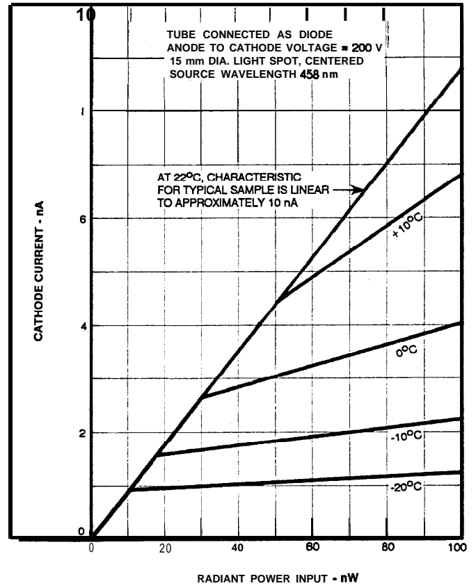
Figure 2: Effect of Temperature on Cathode Responsivity
