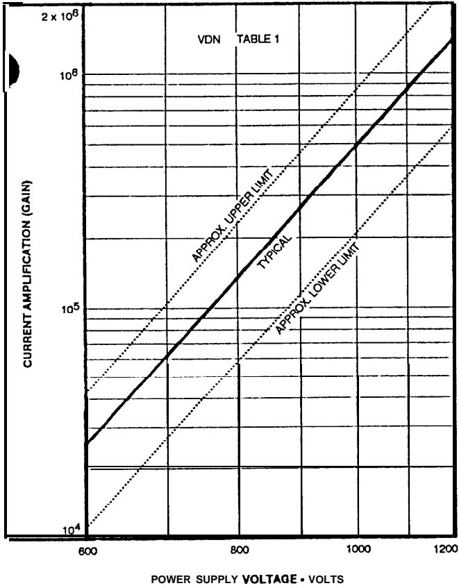
Figure 5: Typical Current Amplification Characteristics
