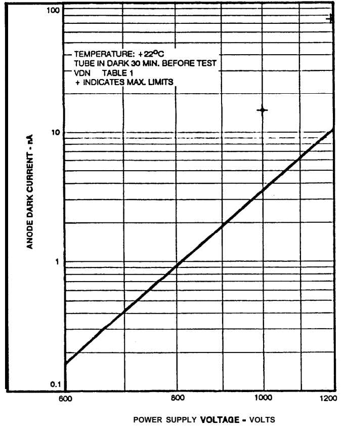
Figure 6: Typical Anode Dark Current Characteristic
