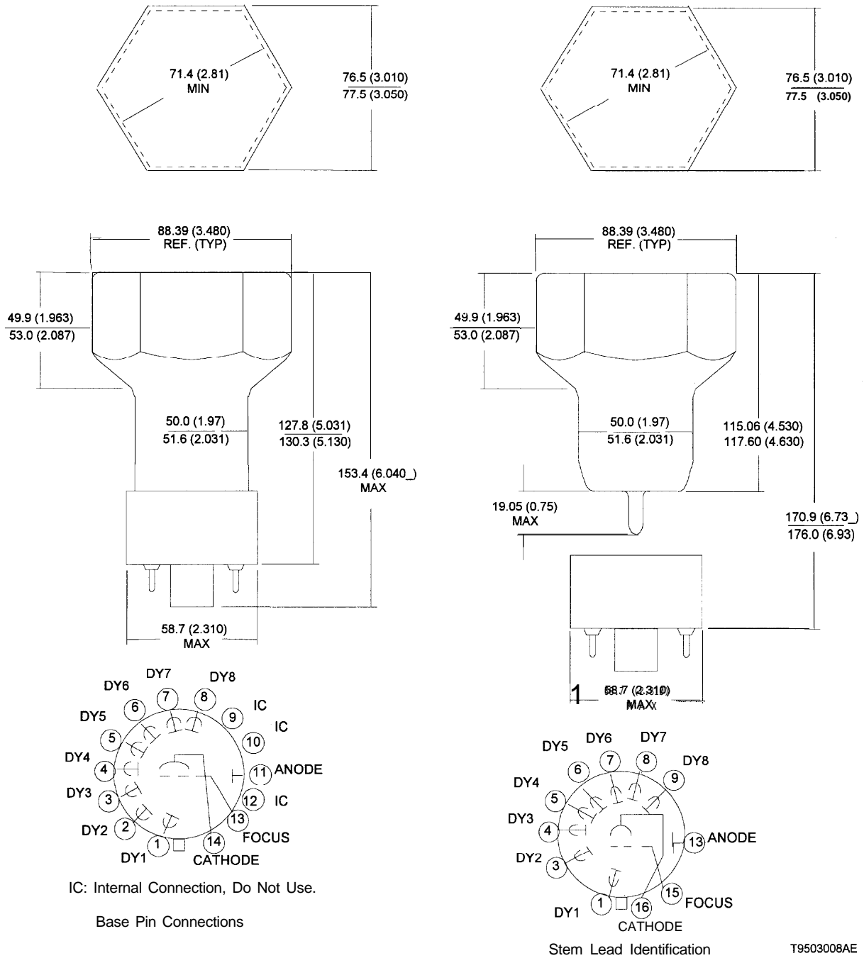
Figure 8: Dimensional Outlines and Basing Diagrams
