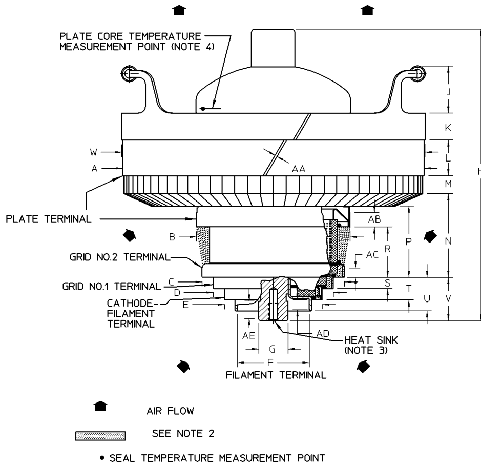
Figure 6 - Dimensional Outline
