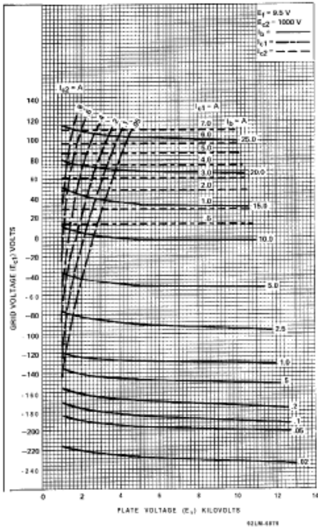
Figure 4 - Typical Constant Current Tube Characteristics @ E_{c2} = 1000 V
