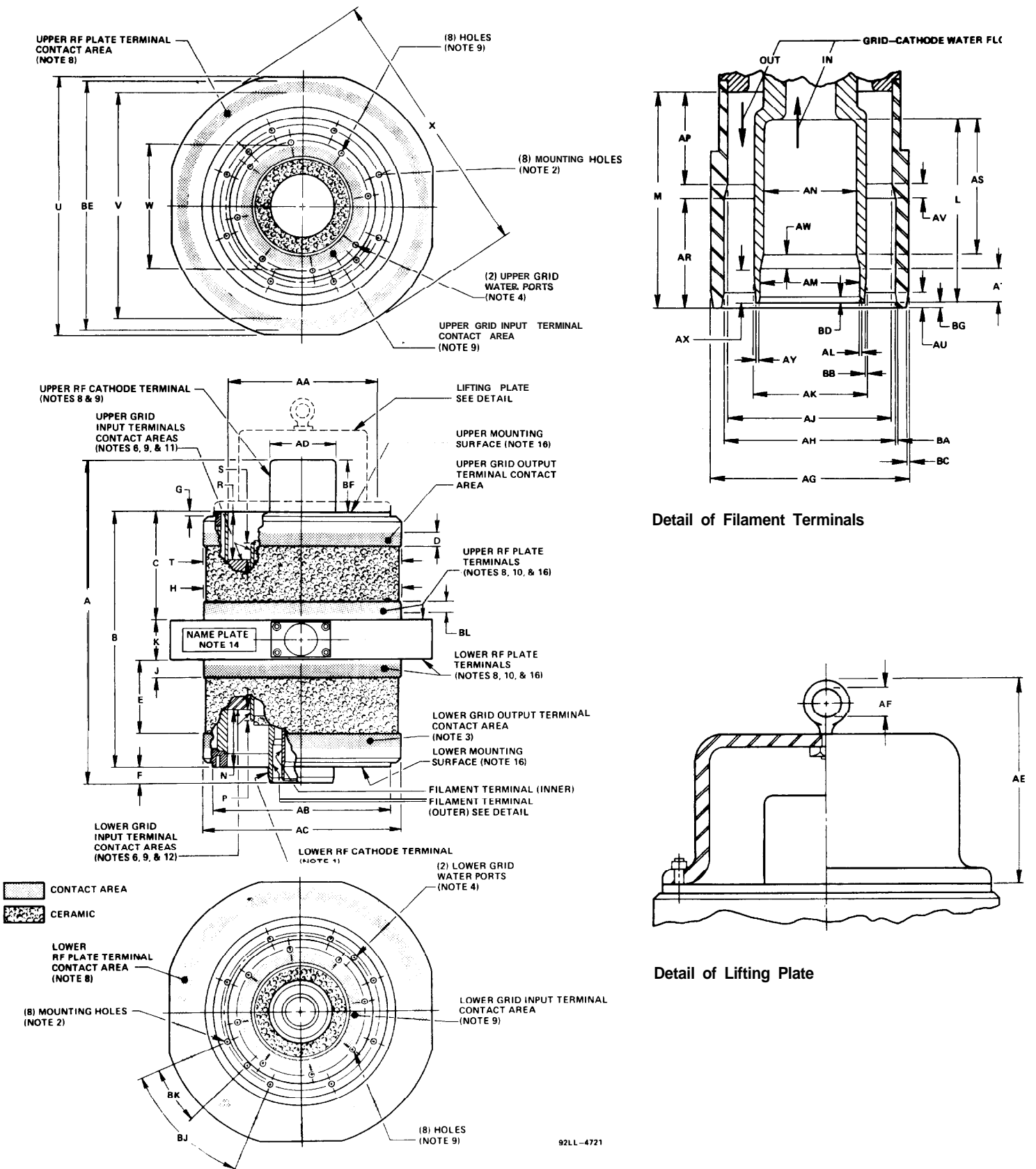
Figure 4 - Dimensional Outline
